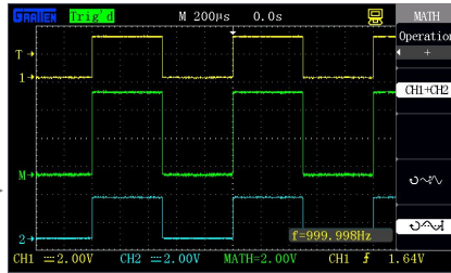
Figure 2-18 MATH Waveform addition
