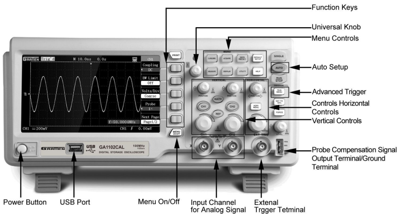
Figure 1-1 Figure of Front Panel controls
