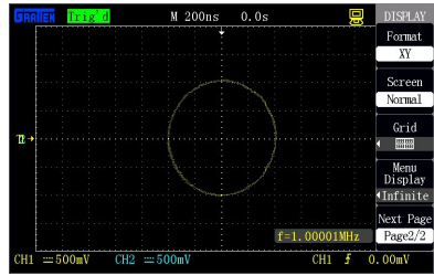
Figure 2-49 X-Y mode
