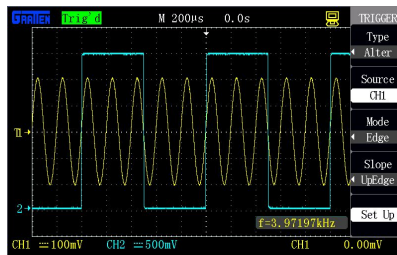
Figure 2-35 Alternating trigger
