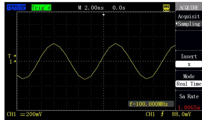
Figure 2-44 Linear interpolation
