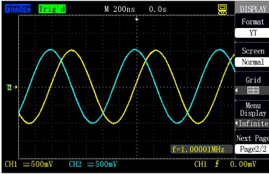
Figure 2-48 Y-T mode
