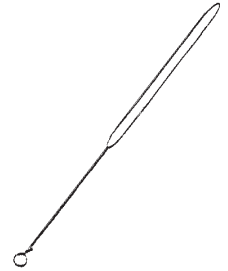
Inoculating loop
