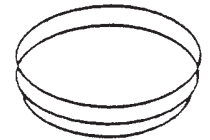
Petri dish
